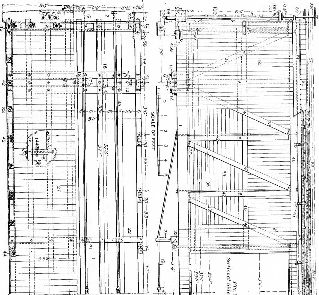
Fig. 233. Half Plan showing Framing.
